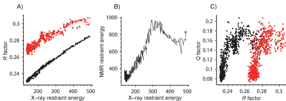
Figure 3. Joint X-ray/NMR refinement and development of quality factors. A) Correlation between R factors and X-ray energy. Black: R_{work} ; red: R_{free} . B) Joint optimization of the restraint energy from the X-ray crystal structure and NMR spectra. C) Correlation between crystallographic R factors and the NMR Q factor. Black: R_{work} ; red: R_{free} . The green dot in panels (B) and (C) indicates the initial structure.
